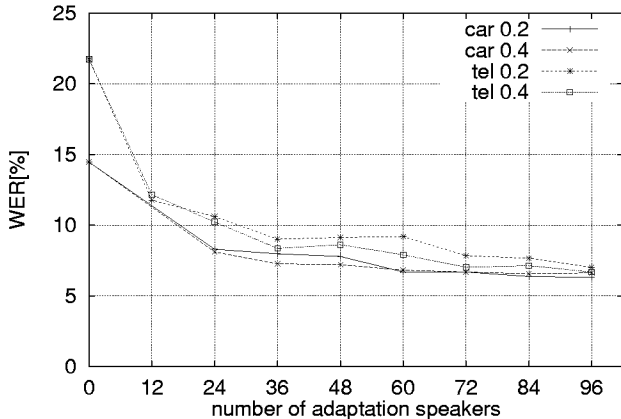
Figure 1: Task-dependent adaptation of car and telephone mono-phone references without online adaptation. The starting point (0 adaptation speakers) is given by the results in Table 1. The numbers behind the environment represent the MAP adaptation factor \alpha .
