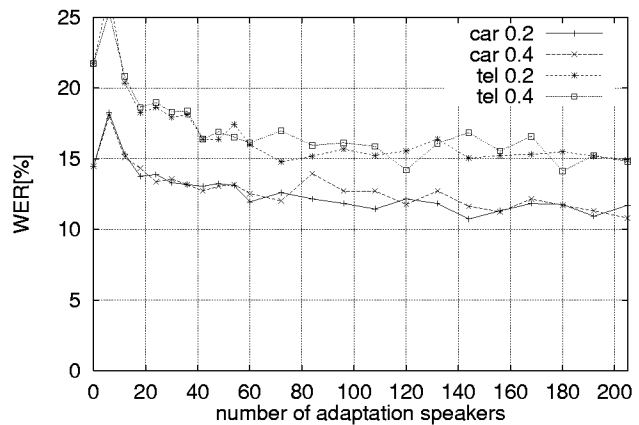
Figure 2: Task-independent adaptation of car and telephone mono-phone references without online adaptation (figures = MAP alpha). The starting point (0 adaptation speakers) is given by the results in Table 1. The numbers behind the environment represent the MAP adaptation factor \alpha .
