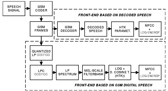
Figure 1: Parameterization procedures.
