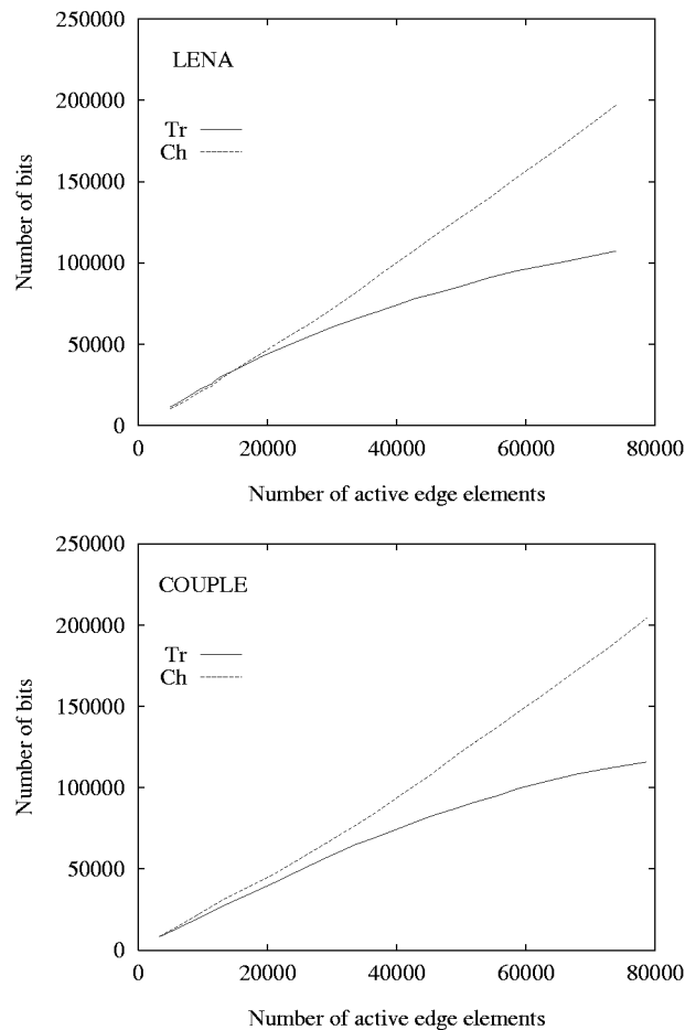
Figure 8: Plots of the number of bits, as a function of the number of active edge elements, required to encode several boundary maps of the “lena” (top) and “couple” (bottom) images. “Tr” refers to the JBIG-based method of transition points, whereas “Ch” denotes the method of differential chain-coding.
