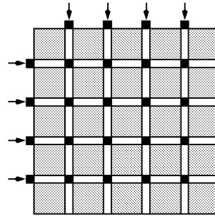
Figure 1: Location of edge elements (white rectangles) and nodes (small black squares). Nodes marked by arrows are called “starting nodes”. Shaded squares indicate pixel positions.
