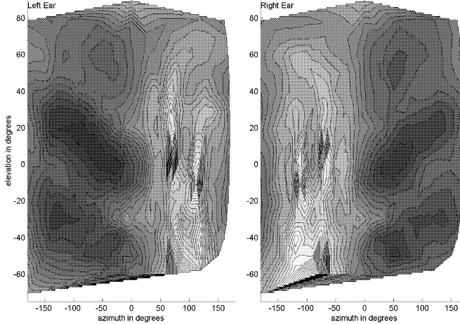
Figure 1. Frequency bin 25/512, 2344-2441 Hz
