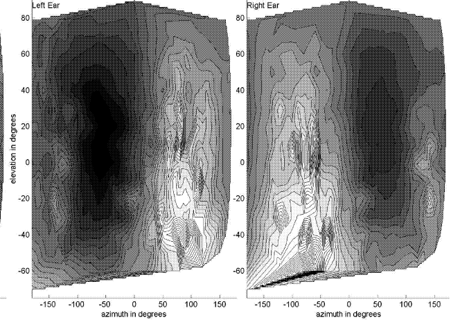
Figure 2. Frequency bin 50/512, 4785-4883 Hz
