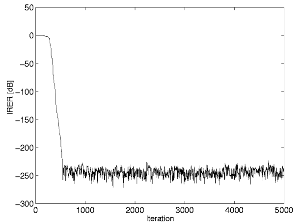
Figure 5: convergence property of IRER( h_2 )
