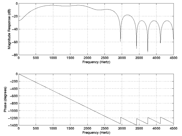
Figure 4: frequency response of the channel
