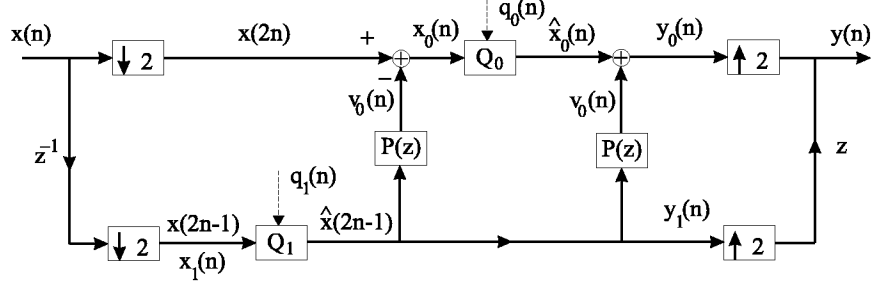
Figure 2: The MINLAB coder.
