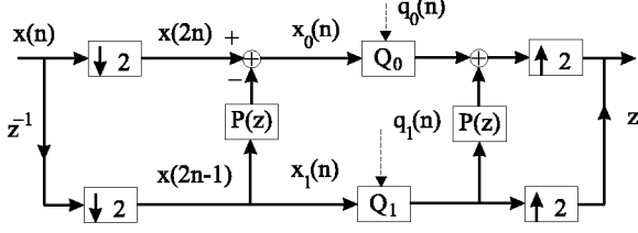
Figure 1: Conventional subband coder using ladder.
