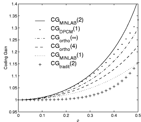
Figure 4: Coding gain for MA(1) process.
