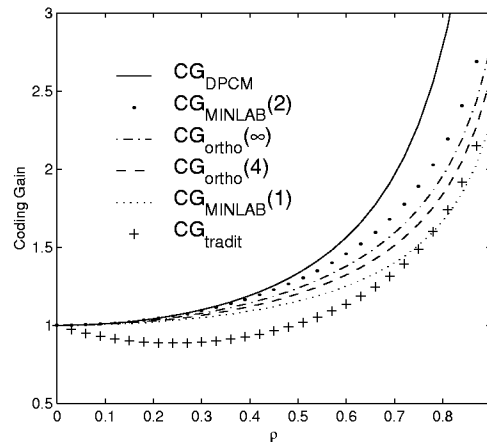
Figure 3: Coding gain for AR(1) process.
