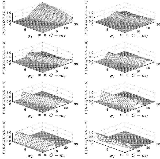
Figure 1: The RXQUAL probability function.
