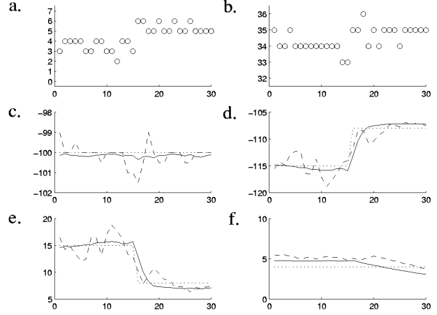
Figure 2: Estimation when there is an abrupt change in the true m_I . Above are the estimated values (dashed) plotted together with an average over several estimations (solid) and the true values (dotted). Measurement reports: a) RXQUAL and b) RXLEV. Estimated parameters: c) Carrier, C , d) Mean interference, m_I , e) C/I , C - m_I , f) Std.dev., \sigma_I .
