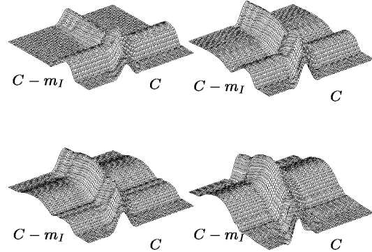
Figure 3: The shape and peak position of the likelihood function changes, when the value of m_I changed abruptly. The maximum of this function is seen to move in the (C - m_I) -direction. The \sigma direction has been eliminated by selecting the true value.
