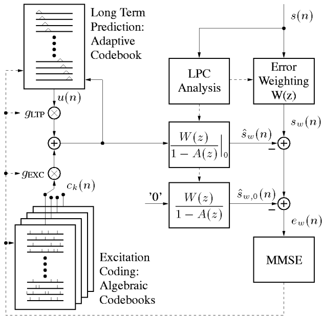
Figure 1: Block diagram of the VR-CELP speech encoder
