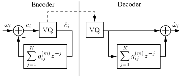
Figure 2: Memory based LSF vector quantization
