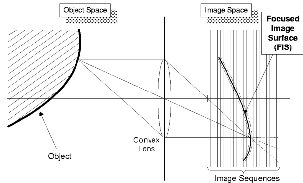
Figure 1. Focused Image Surface in Image Sequences.
