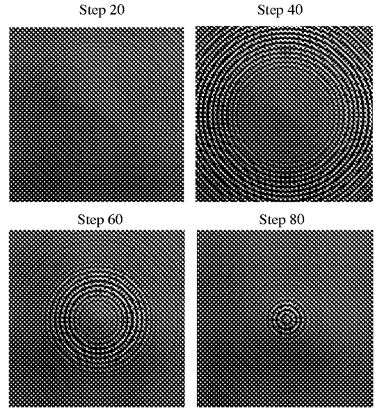
Figure 5. Simulated cone images.
