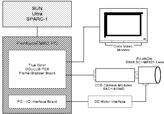
Figure 3. KACS: K-JIST Active Camera System.
