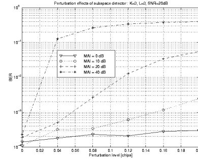
Figure 3: Sensitivity of the subspace detector to the perturbation of delay estimation errors.
