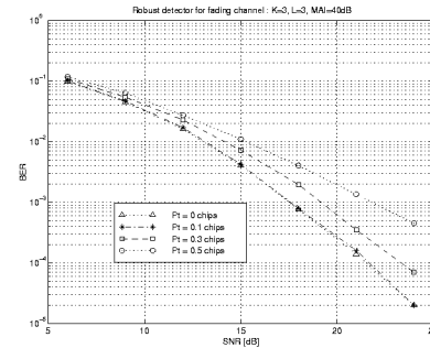
Figure 4: Performance of the robust detector to the perturbation of delay estimation errors.
