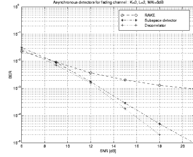
Figure 1: Performance comparison of the asynchronous detectors in a fading channel under perfect power control.
