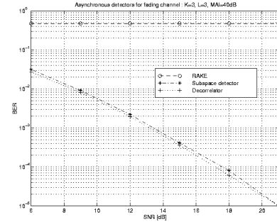
Figure 2: Performance comparison of the asynchronous detectors in a fading channel when MAIs are equal to 40dB.
