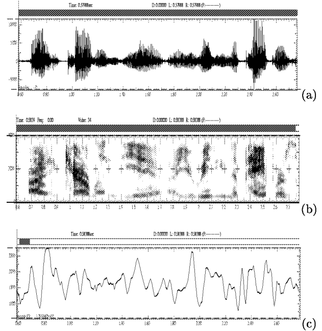
Figure 1. a) waveform, b) wideband spectrogram, c) Jensen Difference values, all for a typical sentence.
