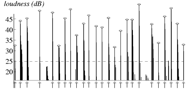
Figure 3. The loudnesses of onsets as a function of their time. The genuine onsets can now be quite easily discerned.
