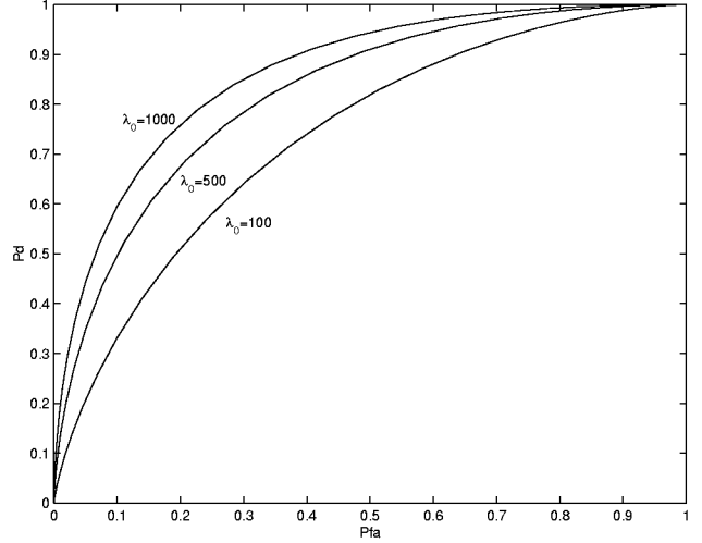
Figure 2: ROC curves for the NPD. p = 1 , a_1 = 0.2 , N - r = 10 and (\lambda_0 = 1000, \lambda_1 = 900) , (\lambda_0 = 500, \lambda_1 = 450) , (\lambda_0 = 100, \lambda_1 = 90) .
