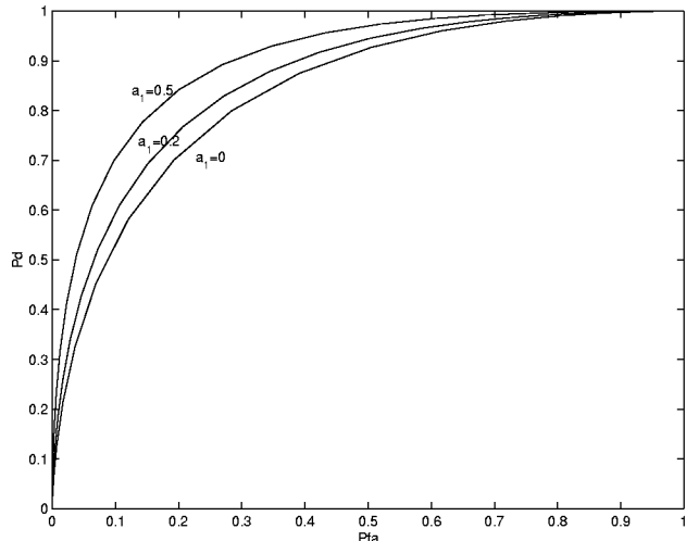
Figure 3: ROC curves for the NPD. p = 1 , N - r = 10 , \lambda_0 = 1000 , \lambda_1 = 900 , and a_1 = 0, 0.2, 0.5 .
