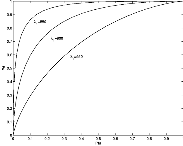
Figure 1: ROC curves for the NPD. \lambda_0 = 1000 , p = 1 , a_1 = 0.2 , N - r = 10 and \lambda_1 = 850, 900, 950 .
