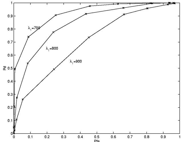
Figure 4: ROC curves for the GLRD. p = 1 , a_1 = 0.2 , N = 512 , r = 412 , \lambda_0 = 1000 and \lambda_1 = 700, 800, 900 .
