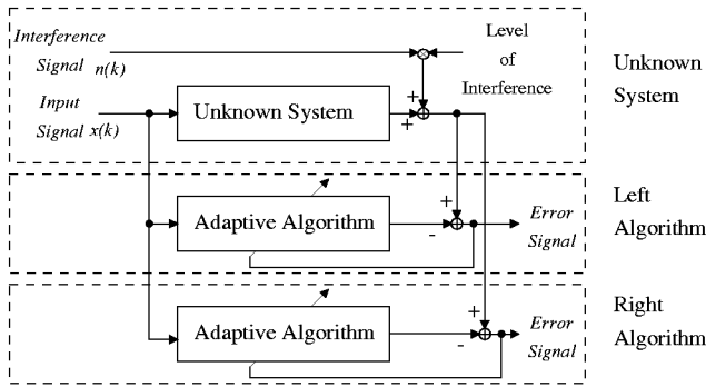
Figure 2. Internal Signal Flow of the Applet.
