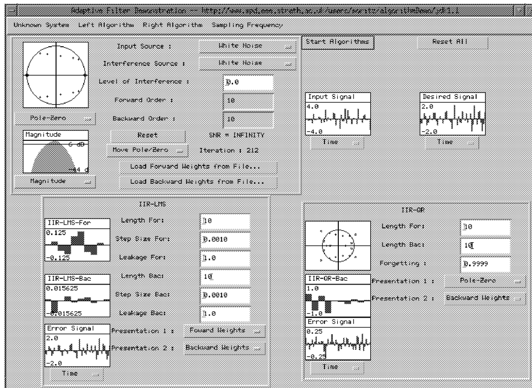
Figure 4. Window simulating two adaptive IIR algorithms and for an IIR unknown system.
