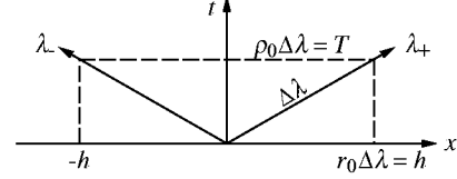
Figure 1: transformation of space and time coordinates
