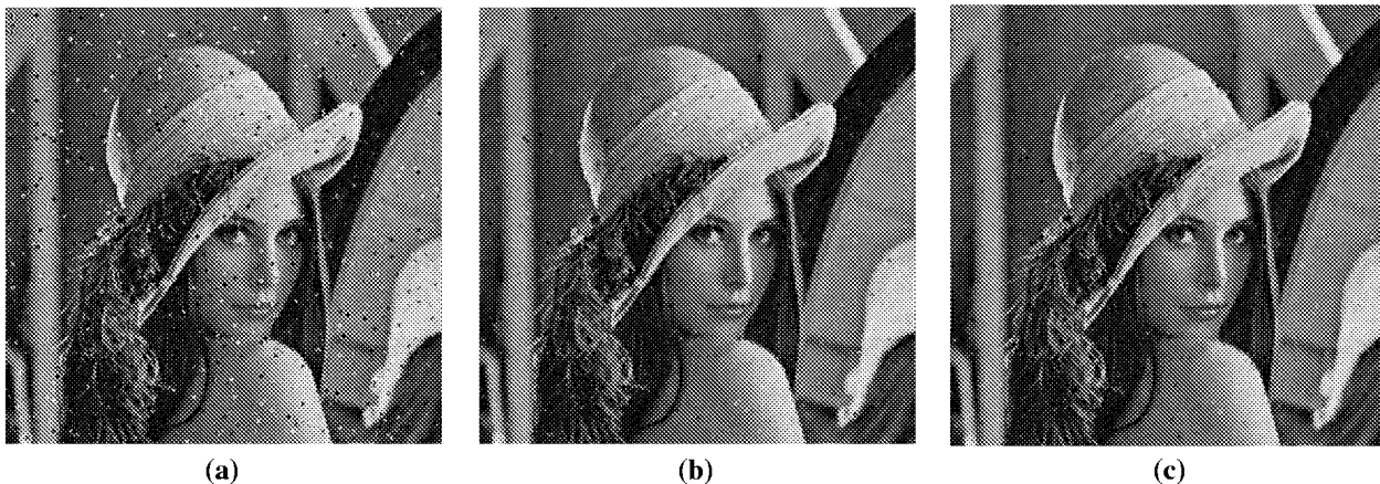
Figure 2: Example of reconstructions. (a) reconstruction from noisy subbands ( P_e = .01 ), without processing (23.6 dB), (b) after processing by the GCP model (28.0 dB) and (c) by the DPQG model (28.6 dB)
