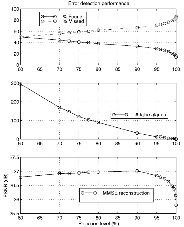
Figure 1: Effect of the rejection threshold on detection and reconstruction performance.
