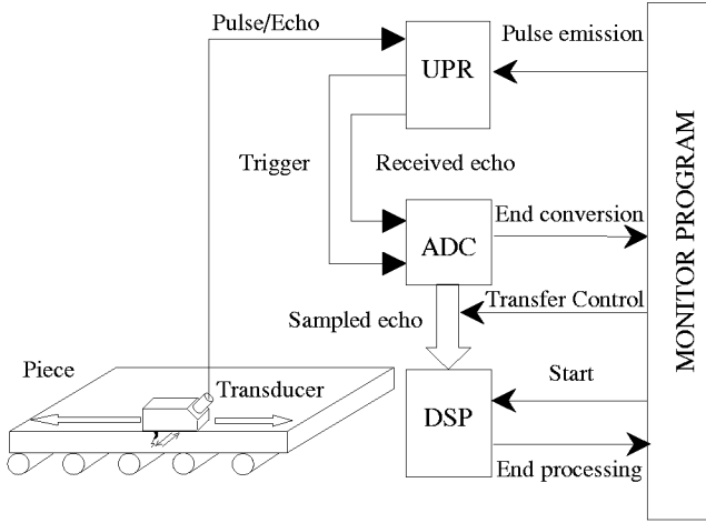
Figure 1. Scheme of the prototype.
