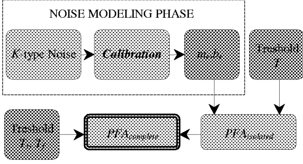
Figure 3. PFA control scheme.
