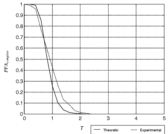
Figure 5. PFA_{complete} for: T_f = 3 T_i = 1 .
