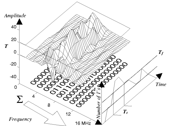
Figure 2. Binarization and double threshold applied to the WVT
