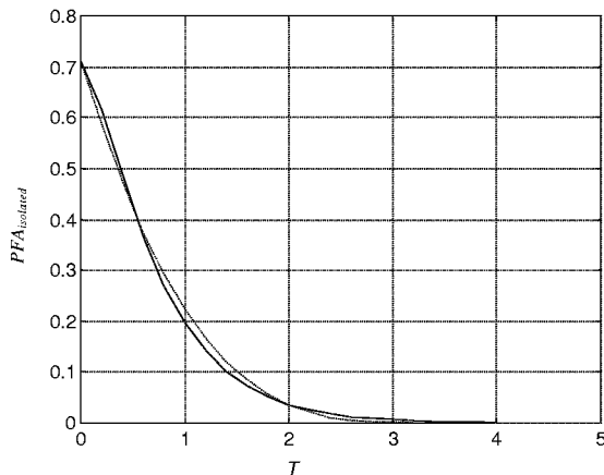
Figure 4. PFA_{isolated} from Eq. 8 (solid line) and from ultrasonic measurements (dotted line).
