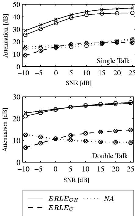
Figure 3: Single Talk (upper diagram) and double talk (lower diagram) results for \hat{H}^{JND} (x) and for H^{LSA} (o), as a function of input SNR.
