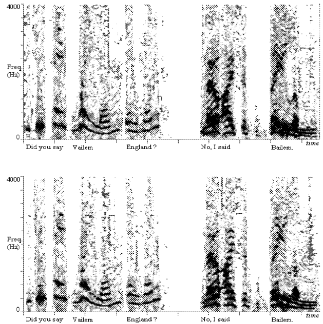
Figure 3: Spectrogram of 4 sec of (female voice) “Did you say Vailem England?” followed by (male voice) “No, I said Bailem”. Top: original. Bottom: Synthetic.
