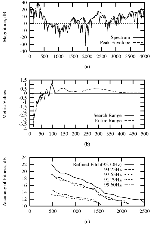
Figure 2: Illustration of pitch refining and spectral decomposition stages; the x-axis is the frequency axis in Hz.
