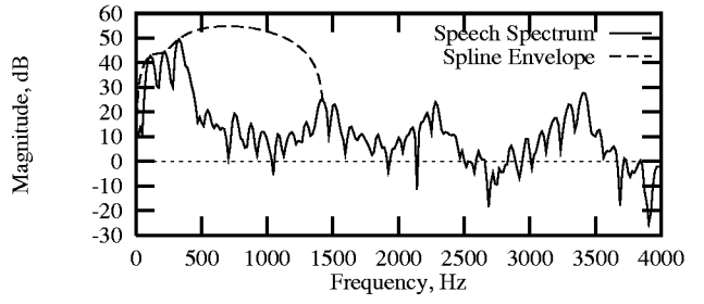
Figure 1: An example of speech spectrum with the periodic energy concentrated under the first 3 harmonics.
