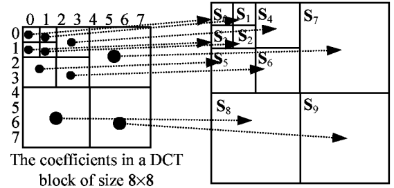
Figure 2. A reordering example for an 8 \times 8 DCT block.
