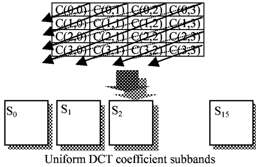
Figure 1. Sorting the coefficients of each 4 \times 4 DCT block in zig-zag order to produce 16 uniform subbands.
