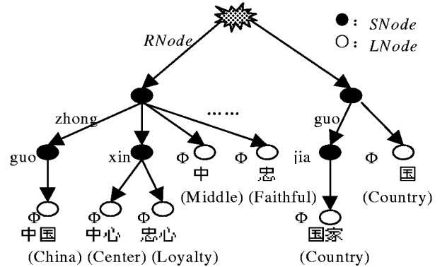
Figure 1. A partial Word Search Tree (WST)
