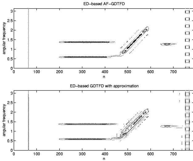
Figure 2: On the top is the AF-GDFTD computed using the first six largest eigenvalues and standard FFT. Below is the result if the additional approximation is performed using the proposed approach.
