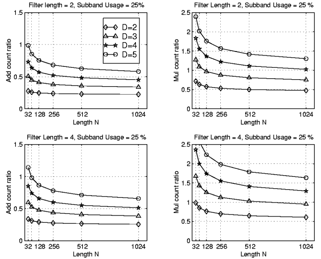
Figure 1: Normalized cost of Eq. 13 versus standard radix-2 FFT followed by (\downarrow 2) .
