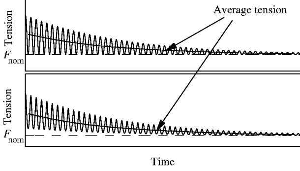
Figure 1. Tension variation of a simulated vibrating string (solid line) for two different plucking points. The tension of the string at rest, F_{nom} , is indicated with a dashed line.
