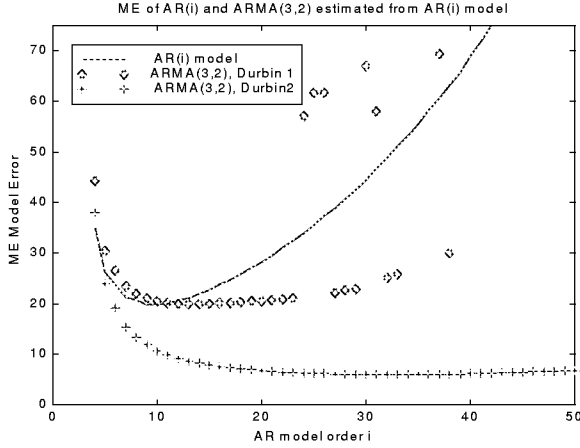
Fig.1 The average Model Error ME of the AR(i) model and two ARMA(3,2) models estimated with Durbin's methods, as a function of the AR model order; 2500 simulation runs, N=100 , true ARMA(3,2) process given in (10).
