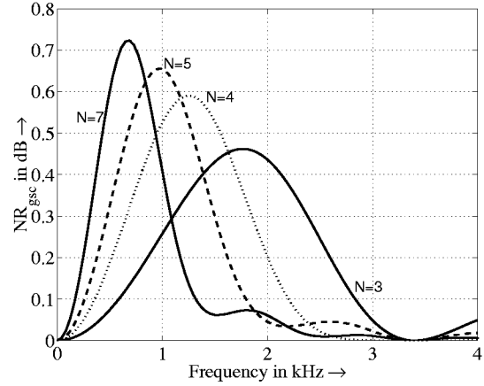
Figure 2: Noise reduction performance in a diffuse noise field for different numbers of microphones ( d = 5cm )
