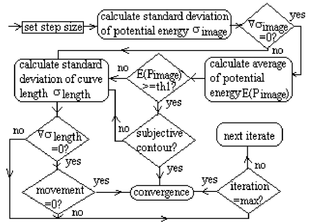
Figure 3. The improved convergent criterion
