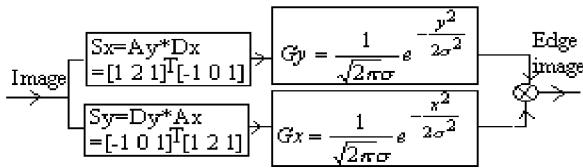
Figure 2. The overall optimal edge detection
