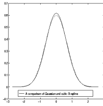
Figure 1: Good approximations of the cubic B -spline (in dotted line) to the Gaussian kernel (in solid line).
