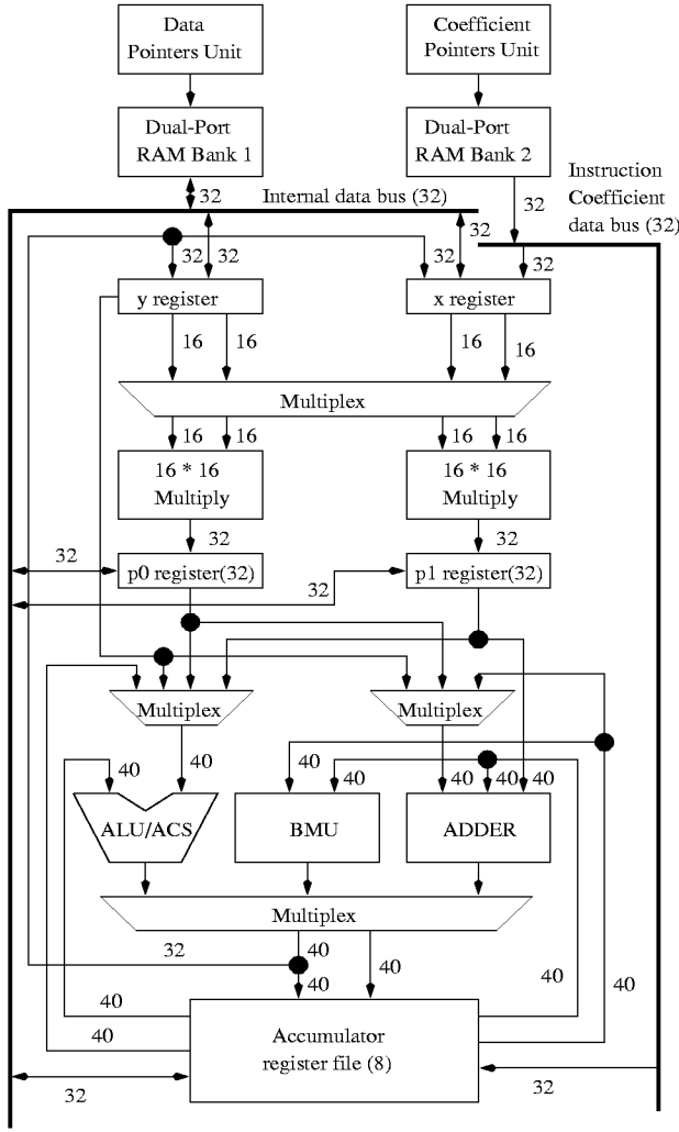
Figure 1: Overview of DSP16000 data path
