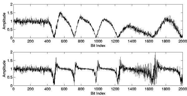
Figure 4: The magnitude of the outputs of the beamformer corresponding to source 2 using only CMA (upper graph) and using the proposed combination (lower graph)
