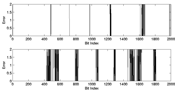
Figure 5: The symbol difference of the output of one beamformer and source 1 (upper graph), and that of the other beamformer and source 2 (lower graph)
