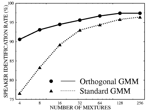
Figure 3 Speaker identification performance with the standard GMM and the OGMM.
