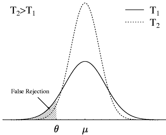
Figure 1: the variance of sentence score decreases with the length of test sentences.
