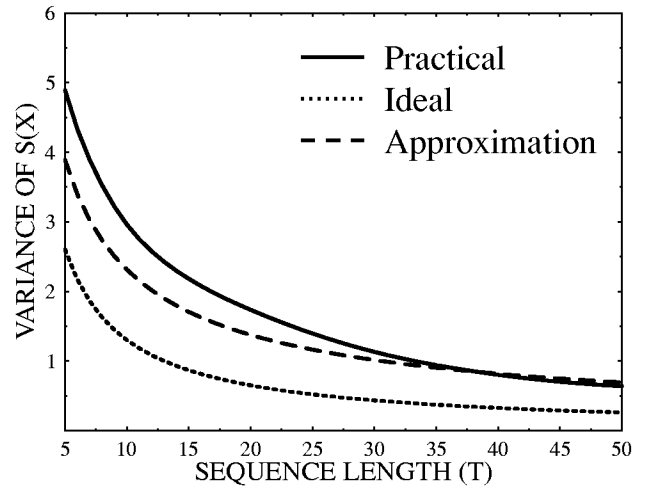
Figure 2: Variance of the sentence score with the length of test sentences in frames. The dashed curve is an approximation to the practical curve.
