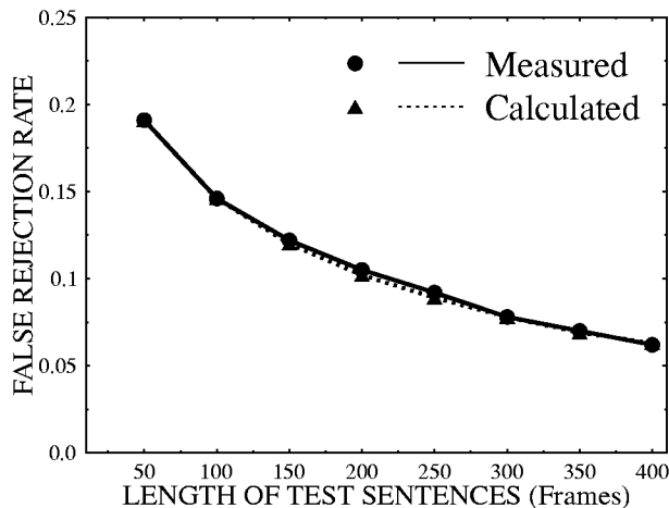
Figure 3: The false rejection rate obtained from the verification experiment and calculated by the proposed method.
