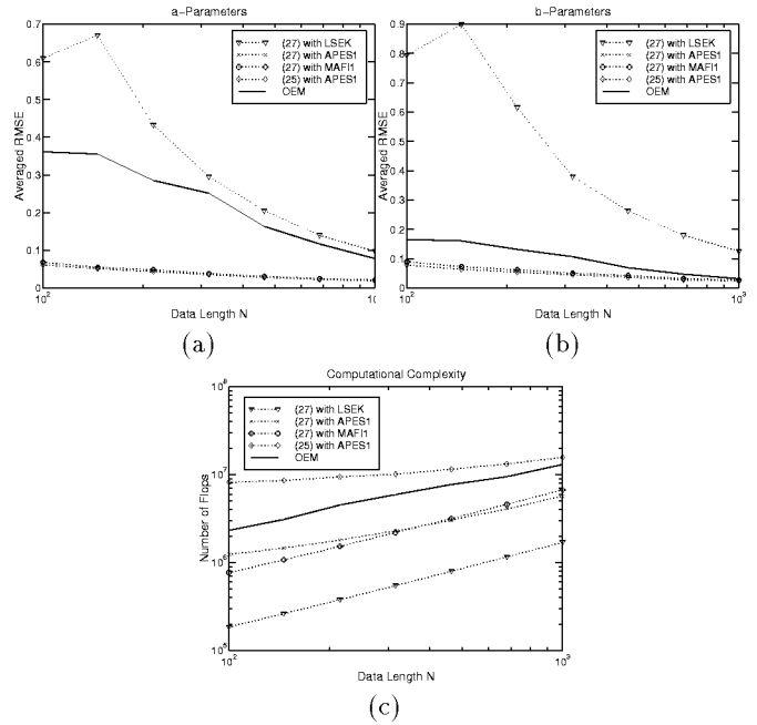
Figure 2. Averaged RMSEs and the number of flops versus N . (a) RMSE of a -parameters. (b) RMSE of b -parameters. (c) Number of flops.
