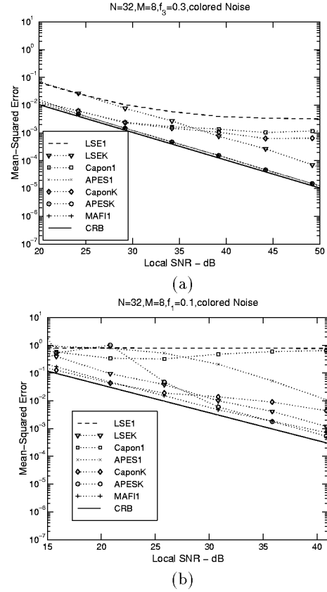
Figure 1. Empirical MSEs and the CRB versus local SNR. (a) \alpha_3 . (b) \alpha_1 .
