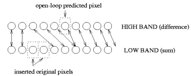
Figure 2: MC Temporal Analysis for TSB and TSB-MCP
