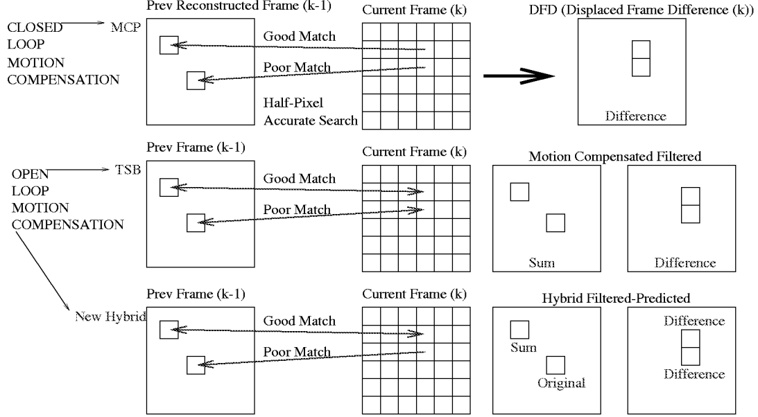
Figure 4: MCP, TSB, and Adaptive TSB-MCP
