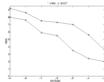
Figure 1: RMS error of TDE, *: CBM, o: SCOT
