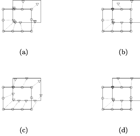
Figure 2: Data centroids after the 1st (a, b) and the 5th (c, d) iterations using (a, c) fuzzy c-means and (b, d) snake sensor models. \bigcirc - model units, \nabla - centroids.
