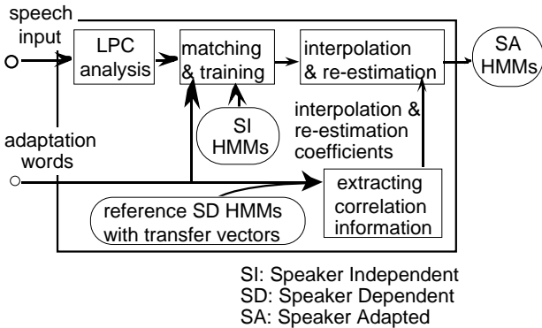
Figure 5: Block-diagram of Speaker Adaptation Algorithm.
