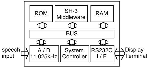
Figure 1: Example of System Architecture
