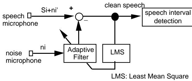
Figure 2: Block-diagram of ANC for Speech Interval Detection
