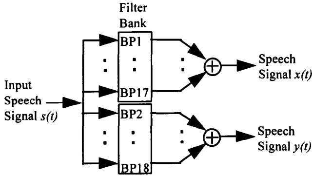
FIGURE 1. Splitting of speech signal using multiple bandpass (BP) filtering. The 3 dB cutoff frequencies of the bands are in kHz.
