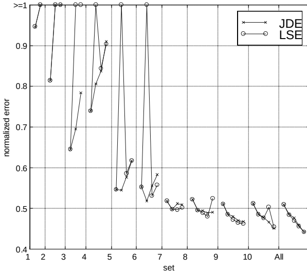
Figure 2: Conversion test errors produced by JDE and LSE after training on different data sets. From left to right within one set, the number of mixtures is 1, 2, 4, 8, and 16.
