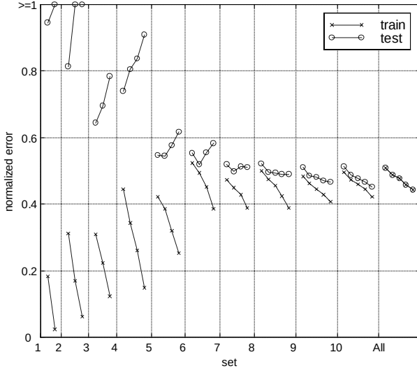
Figure 1: Conversion training and testing errors produced by JDE after training on different data sets. From left to right within one set, the number of mixtures is 1, 2, 4, 8, and 16.
