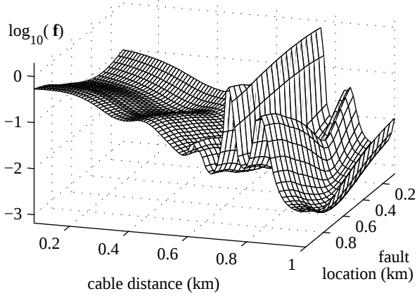
Figure 4: Feature vectors of varying fault locations for a ground fault impedance of 500 \Omega .
