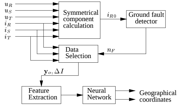
Figure 2: Ground fault detection system.
