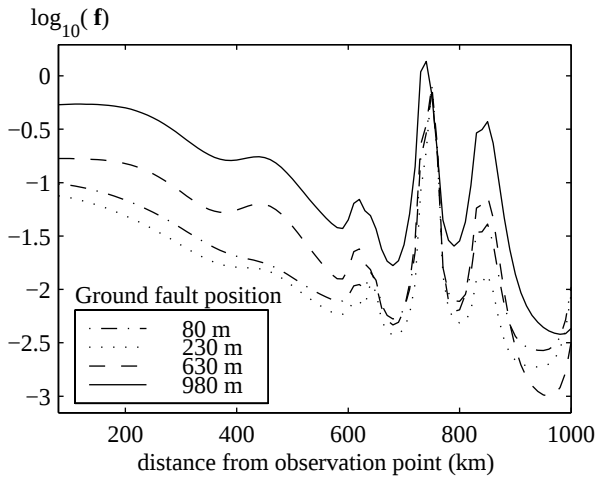
Figure 5: Feature vectors of three fault locations for a ground fault impedance of 500 \Omega .
