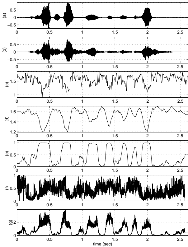
Figure 2: (a) Clean speech signal. (b) Reverberant speech signal. (c) The moving entropy computed from the LP residual of reverberant speech in (b). (d) Interpolated and smoothed version of the entropy function in (c). (e) Gross weight function. (f) Normalised prediction error. (g) Overall weight function.
