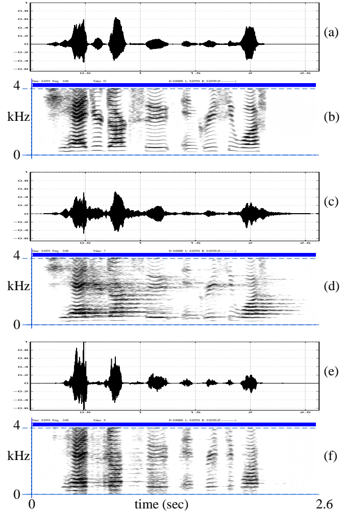
Figure 3: (a) Clean speech. (b) Spectrogram for clean speech. (c) Speech degraded by reverberation. (d) Spectrogram for speech degraded by reverberation. (e) Enhanced speech using gross and fine level weighting of the LP residual. (f) Spectrogram for enhanced speech using gross and fine level weighting of the residual.
