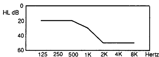
Fig. 6. Target Hearing Loss
