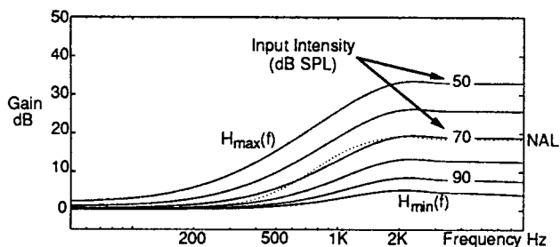
Fig. 4. Continuum Based on Extending NAL
