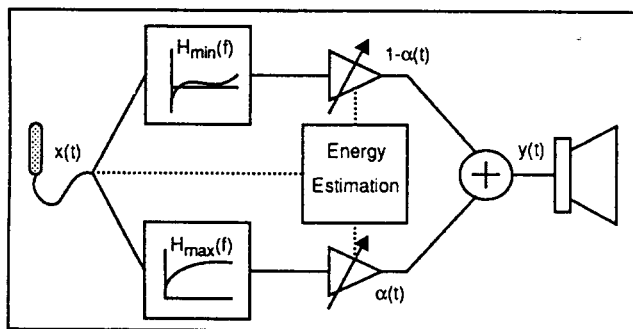
Fig. 2. Filter Mixture Structure
