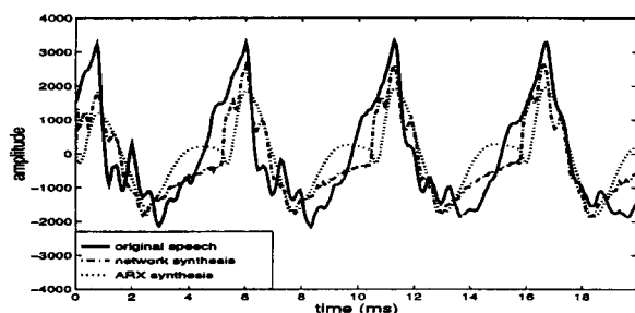
Figure 4: Synthesis for ARX initialisation model ( n_a=10, n_b=9 ) and recurrent network after 3000 epochs of training from the ARX initialisation.
