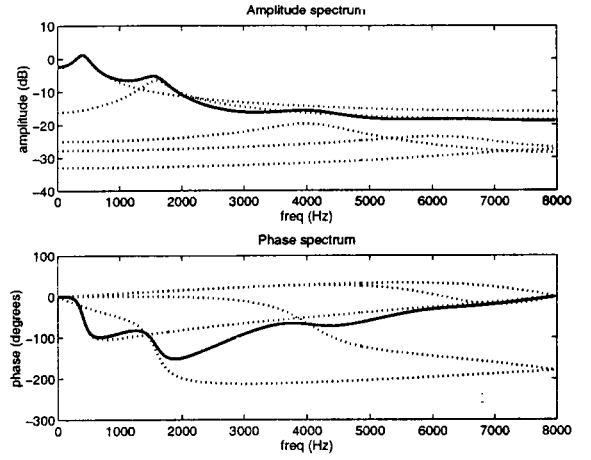
Figure 2: Spectra and formant factors (dotted curves) for a typical ARX model ( n_a = 10 , n_b = 1 ).
