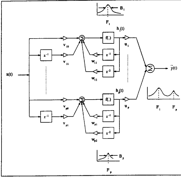
Figure 1: Structure of recurrent network.
