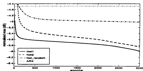
Figure 3: Learning curves for different initialisations. Net1:ARX initialisation ( n_a = 10, n_b = 9 ). Net2:ARX initialisation ( n_a = 10, n_b = 1 ). Net_random:random initialisation ( n_a = 10, n_b = 9 ). ARX:synthesis error for actual ARX model ( n_a = 10, n_b = 9 ).
