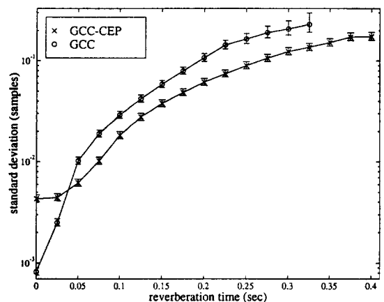
Figure 3: Standard deviation of the non-anomalous time delay estimates versus reverberation time obtained with and without cepstral prefiltering.
