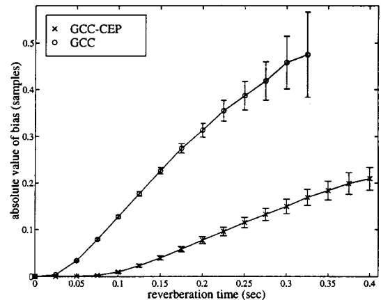
Figure 2: Bias of the non-anomalous time delay estimates versus reverberation time obtained with and without cepstral prefiltering.
