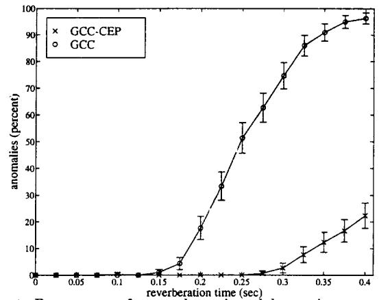
Figure 1: Percentage of anomalous time delay estimates versus reverberation time obtained with and without cepstral prefiltering.
