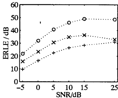
Figure 6: Echo return loss enhancement (ERLE) of two-microphone system in a car: (+) \overline{ERLE\_C(k)} (echo canceller only); (x) \overline{ERLE\_CH(k)} (combined system) with a(k) = 0 ; (o) \overline{ERLE\_CH(k)} (combined system) with a(k) adaptive.
