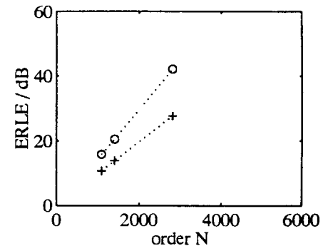
Figure 4: \overline{ERLE}_C(k) and \overline{ERLE}_{CH}(k) as a function of compensator order N ; a(k) adaptive.
