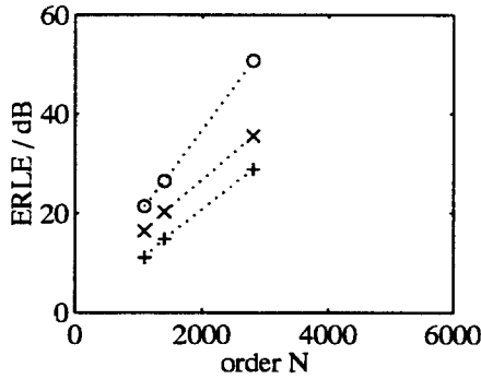
Figure 5: ERLE vs . compensator order of the two-microphone system for an meeting room: (+) \overline{ERLE\_C(k)} (Echo canceller only); \overline{ERLE\_CH(k)} for a(k) = 0 (x) and for a(k) adaptive (o).
