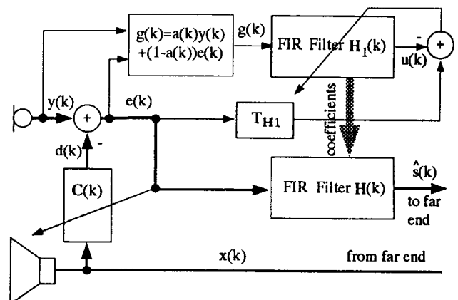
Figure 1: Echo canceller combined with FIR echo attenuator.
