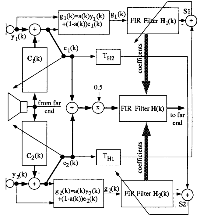
Figure 2: Basic block diagram of the two-microphone coupled filter approach.
