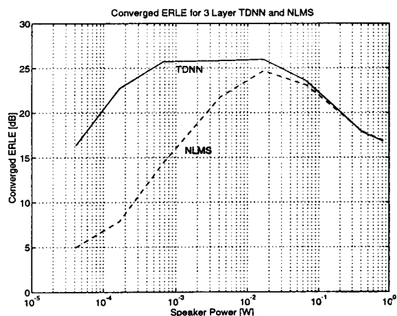
FIGURE 6. Experimental Results. Converged ERLE plot vs. loudspeaker volume using a three layer fully adaptive TDNN. The three layer network (solid line) shows over 10 dB improvement in ERLE at low to medium volumes. The NLMS algorithm (dashed line) is shown for comparison.
