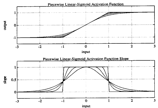
FIGURE 4. Piecewise linear-sigmoid activation function and corresponding delta. The linear section with a value of \pm 0.2 gave the best results in this study.
