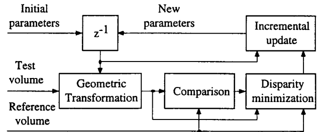
Figure 1: Outline of the registration algorithm
