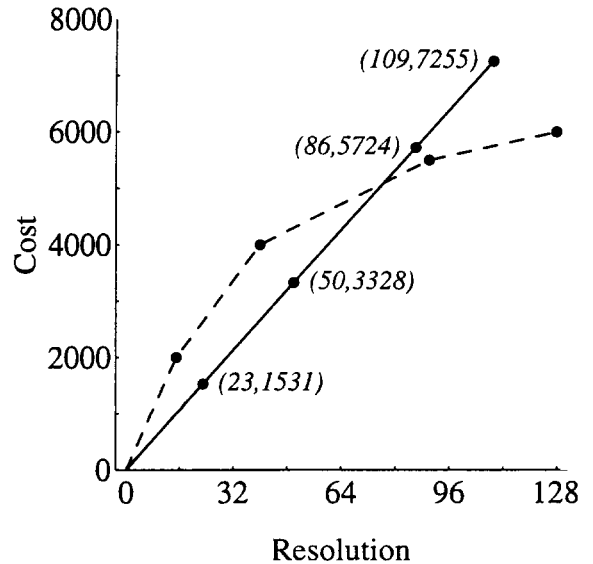
Figure 3: Refinement path in frequency resolution of algorithm (solid line) designed to approximate a given path (dashed line). Each point indicates the output quality after a particular stage is completed and is labeled with the cumulative cost incurred through that stage in complex additions.
