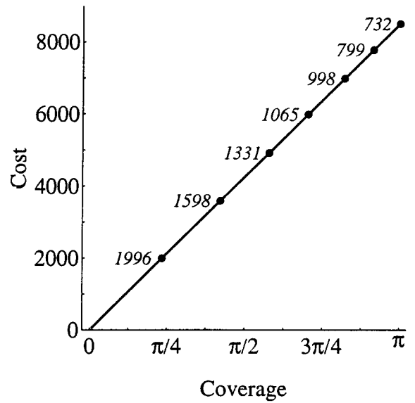
Figure 2: Refinement path in frequency coverage of algorithm designed with exponentially decreasing cost increments. Each point indicates the output quality after a particular stage is completed and is labeled with its associated cost increment in complex additions.
