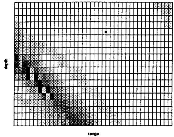
Figure 5: Source at (5 Km, 250 m).
