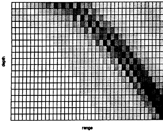
Figure 3: Source at (7 Km, 200 m).
