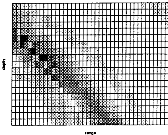
Figure 4: Source at (5 Km, 150 m).
