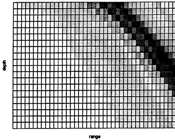
Figure 2: Source at (7 Km, 150 m).
