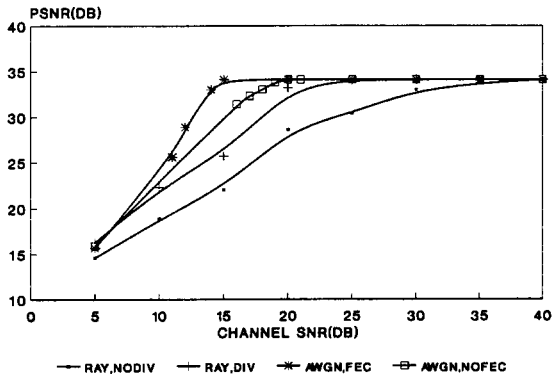
Figure 5: 16QAM PSNR versus channel SNR performance over various channels
