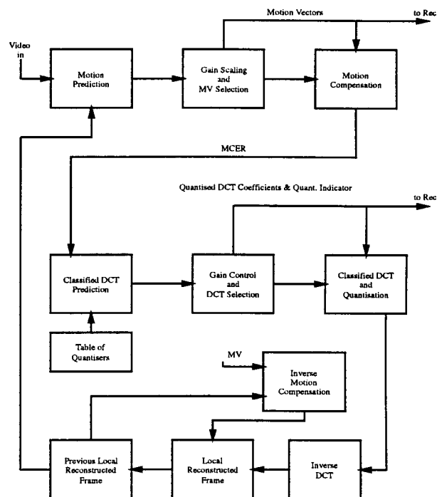
Figure 1: Encoder Schematic
