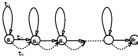
Figure 3: HMM Topology
